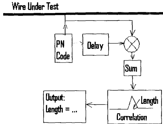
Fig. 7 Sequence (STDR) Test System. For SSTDR, the input signal is a sine wave modulated PN code
