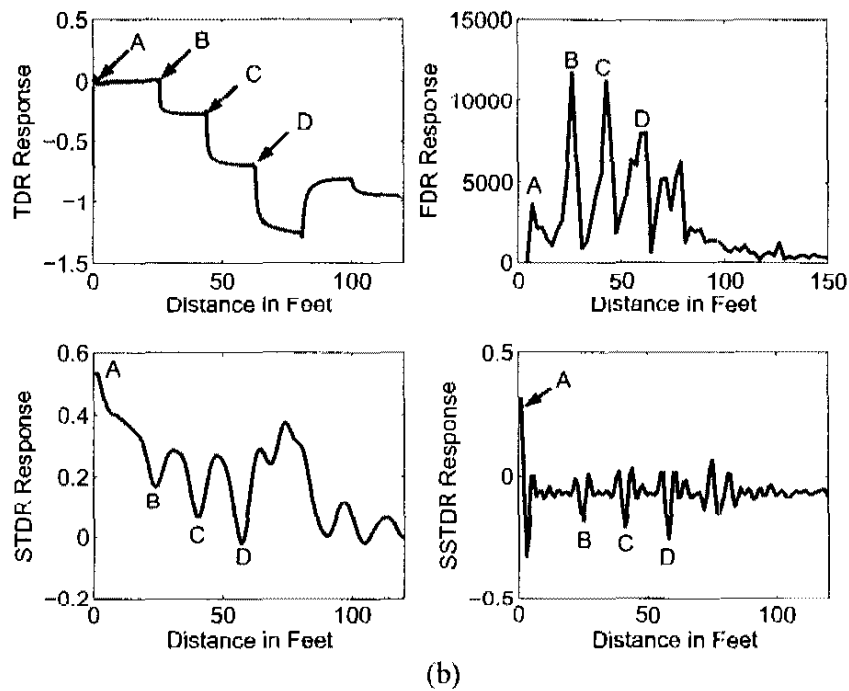
Fig. 3 (a) Network topology, (b) Reflectometry test signals of network shown (a) with TDR, FDR (MSR/SWR), STDR, SSTDR
