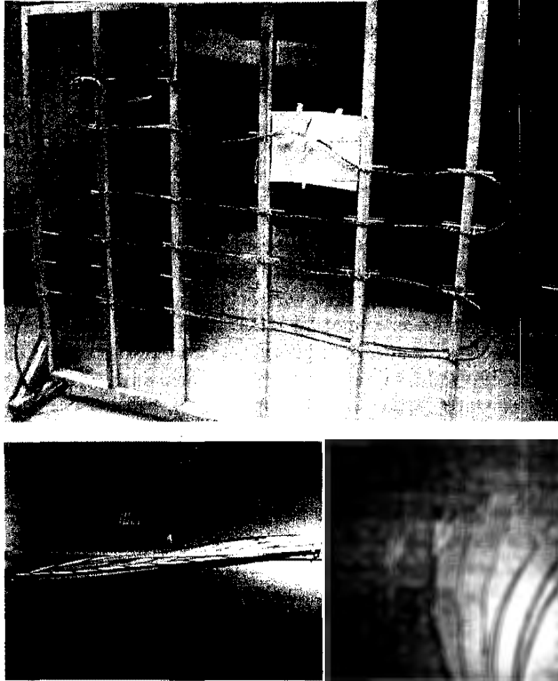
Fig. 9 Test bed, wire bundles and wire types
