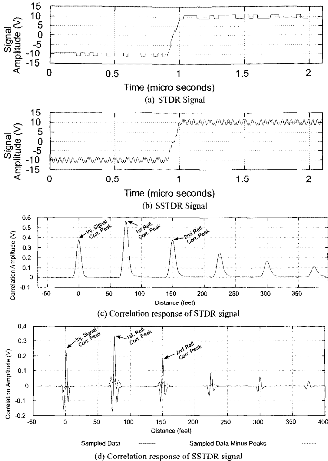
Fig. 8 STD and SSTDR signal added to a 10 V RMS signal at 30 MHz. The S/SSTD signals are a Maximum Length (ML) Code 1V RMS at 58 MHz, with a 58 MHz sine wave modulation in the case of SSTDR. The magnitude of the S/SSTD signals can be much smaller than shown here, depending on the signal on the wire. (a) STD Signal (b) SSTDR Signal (c) Correlation response of STD signal (d) Correlation response of SSTDR for a 75 foot wire (RG58 coax) that is open circuited on the end. From Furse, et al. (2005), Smith (2003).
